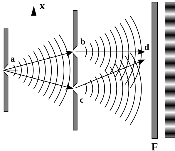
Figure 1: Young's interference.
