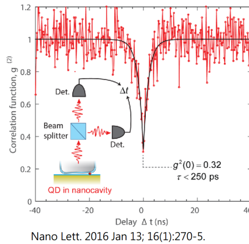
Figure 5: Experiment of single photon measurement.
