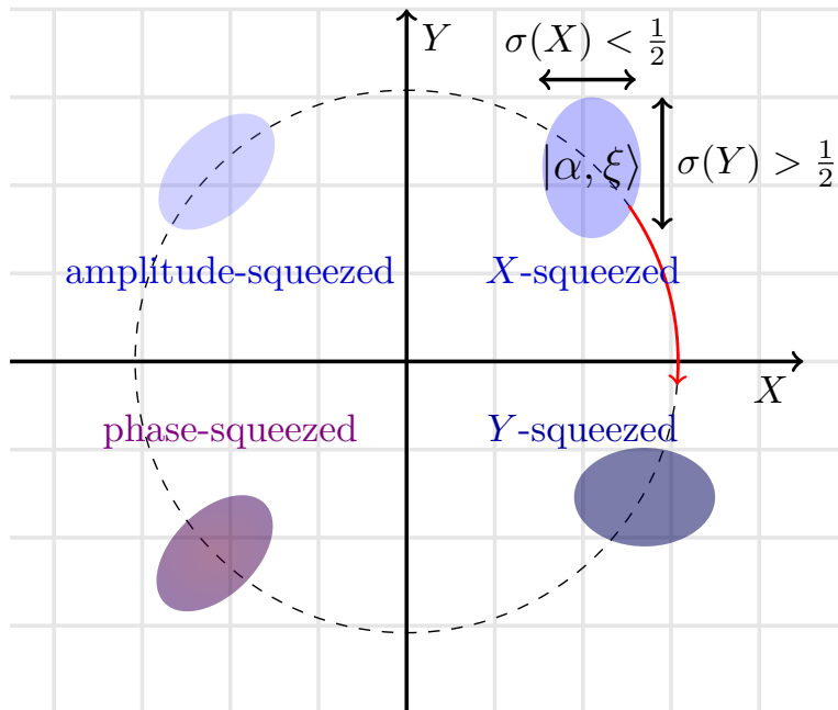
Figure 6: Squeezed States.
