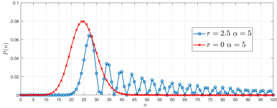
Figure 8: Photon counting of squeezed states. \alpha = 5
