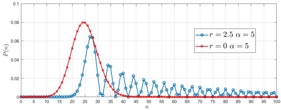
Figure 8: Photon counting of squeezed states. \alpha = 5
