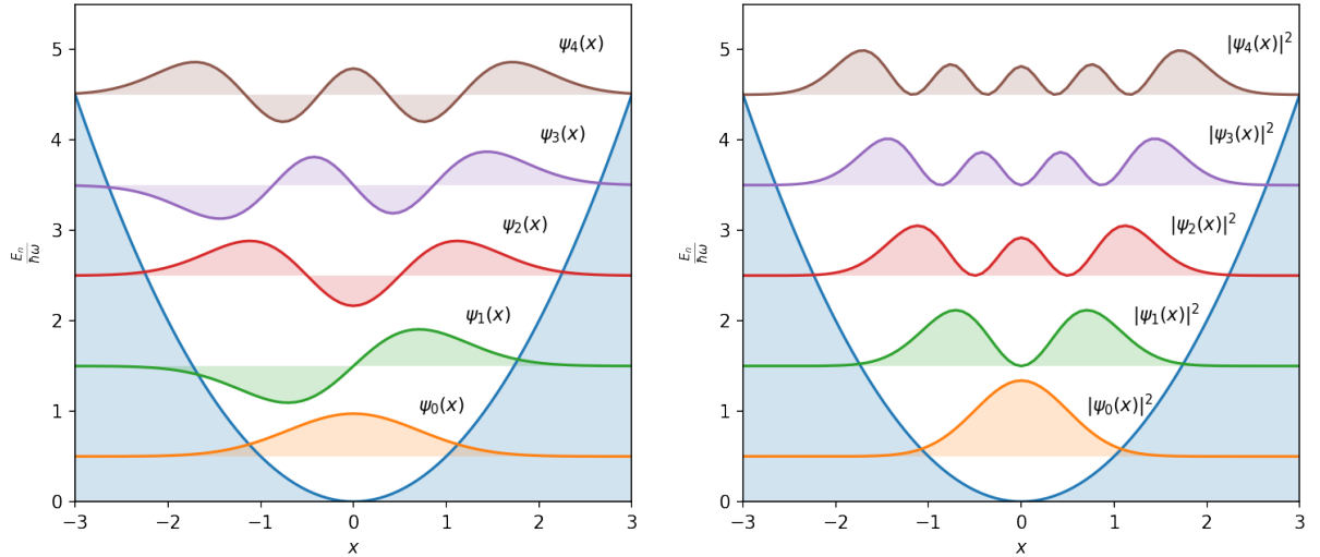
Figure 2: Wavefunction \psi_n(x) .
