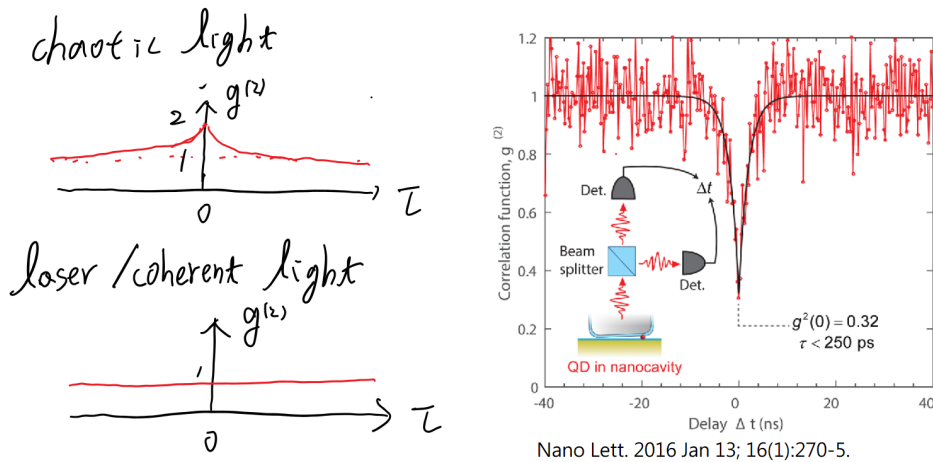
Figure 3: g^{(2)}(\tau) of various photon ensembles.
