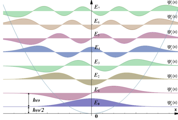
Figure 2: Wavefunction \psi_n(x) .
