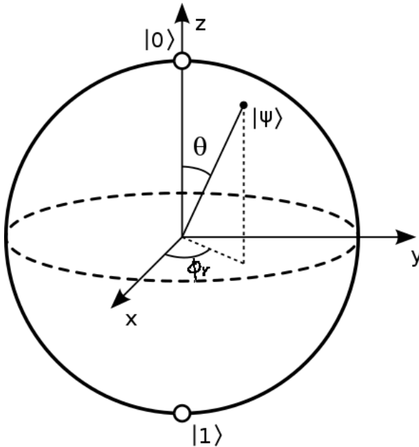
Figure 1: Bloch sphere.
